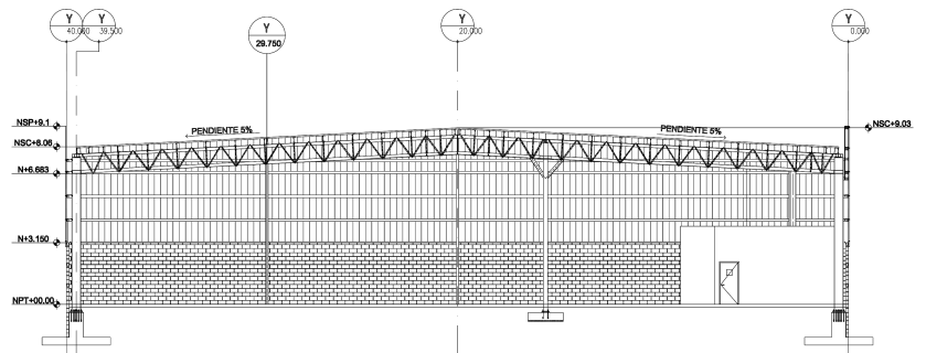
BUILDING SECTION
